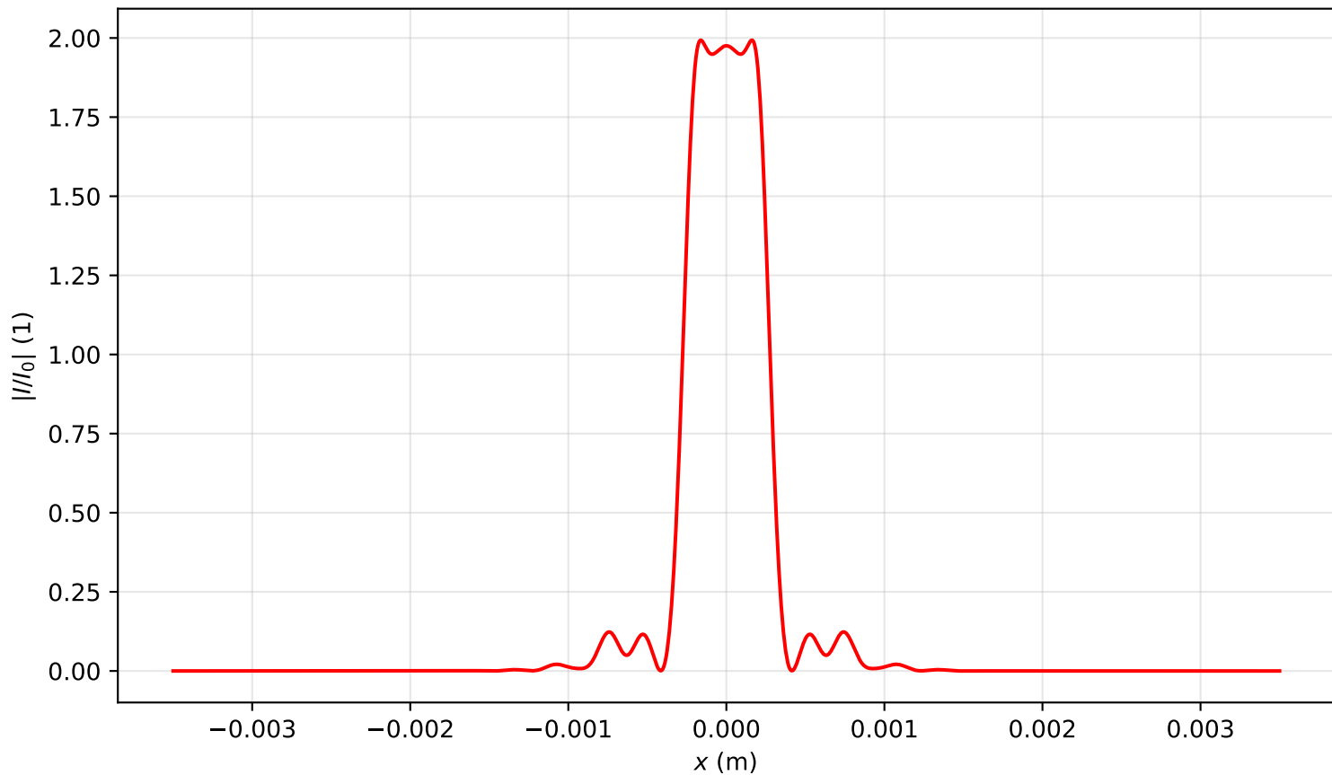
Intensity profile I(x, y = 0, z = 0.716)/I_0 , P_{in}=7.5P_{cr} , artificial time
